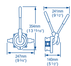
Bulkhead/Removable Handle BP9021 Plan View Side View
